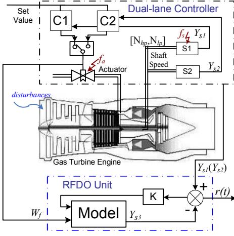
Fig. 1. Dual-lane in modern gas turbine engines.
