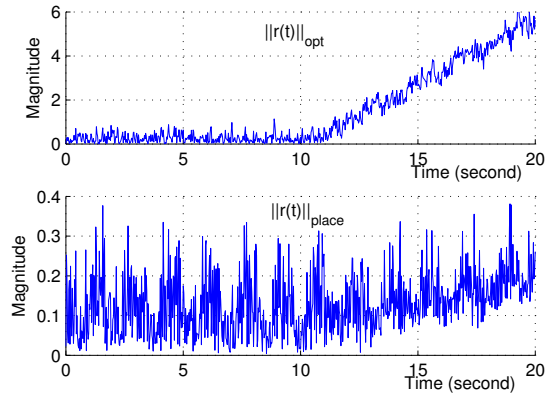
Fig. 6. Residuals of K_{opt} and K_{place} in the case of incipient sensor faults
